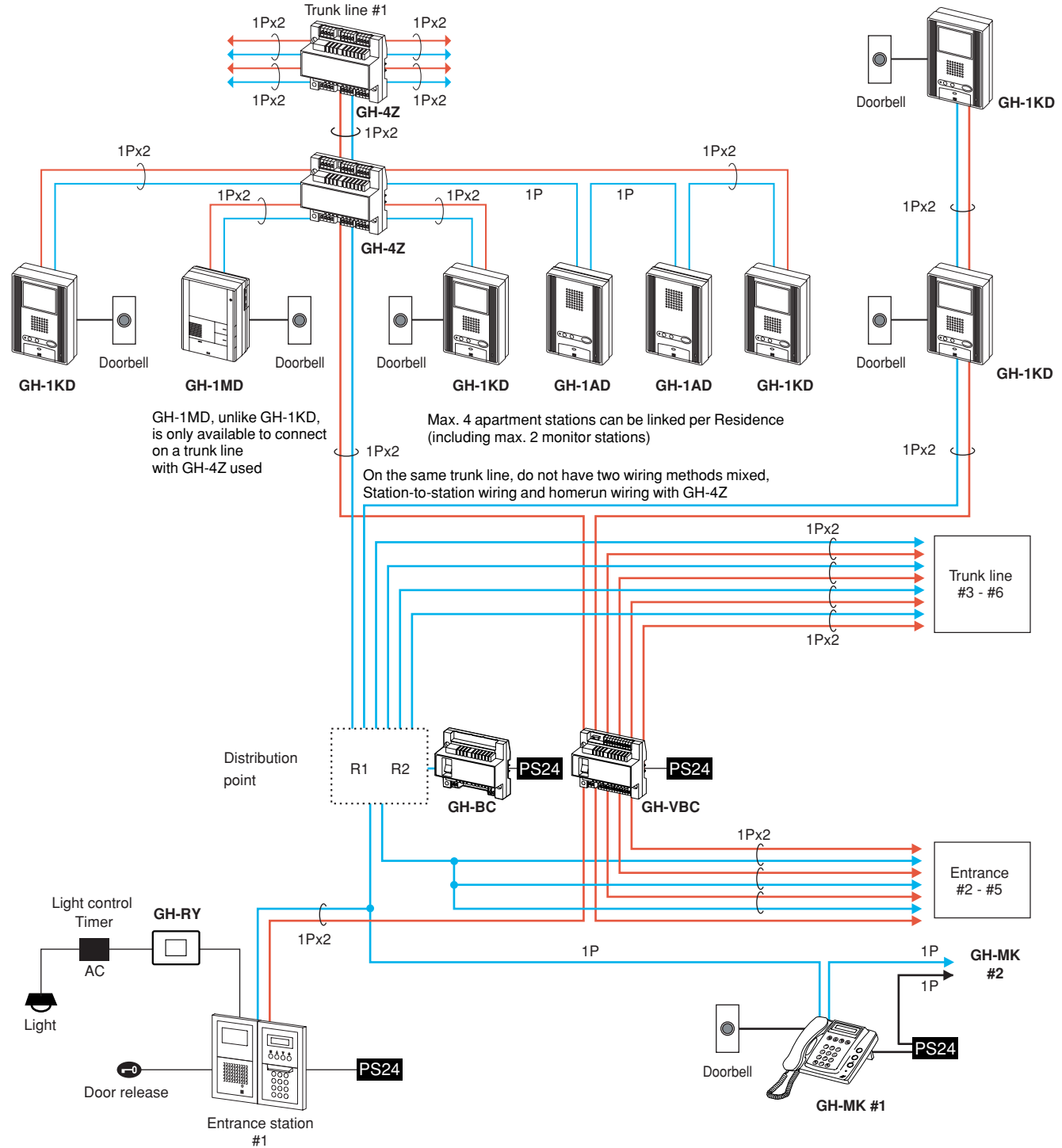
Homerun wiring with GH-4Z
